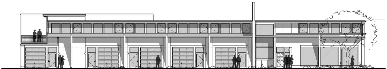
SOUTH ELEVATION
